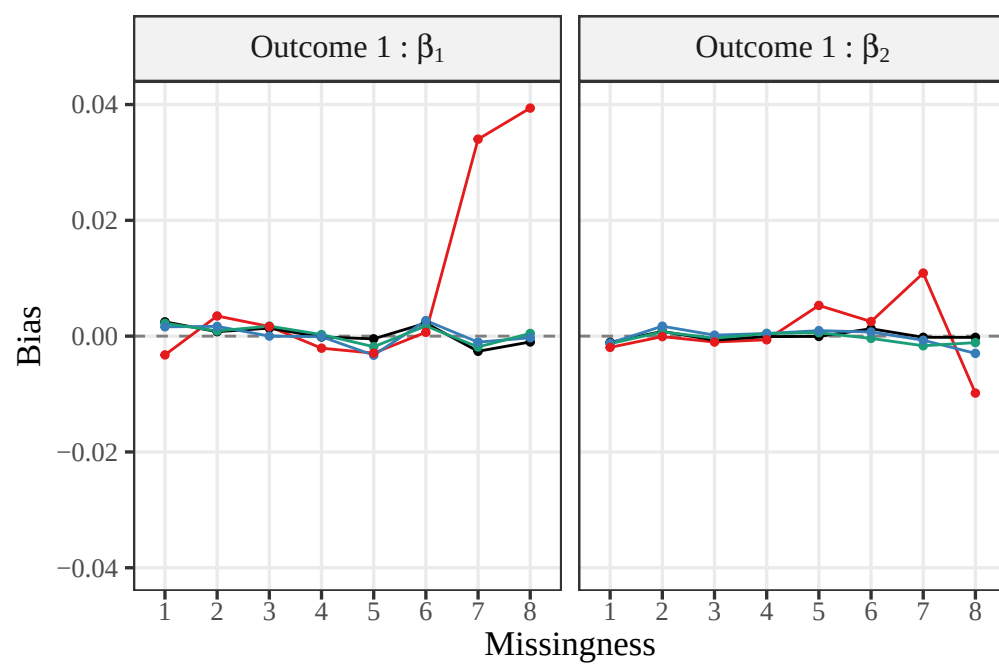
Variance Comp: Bias
