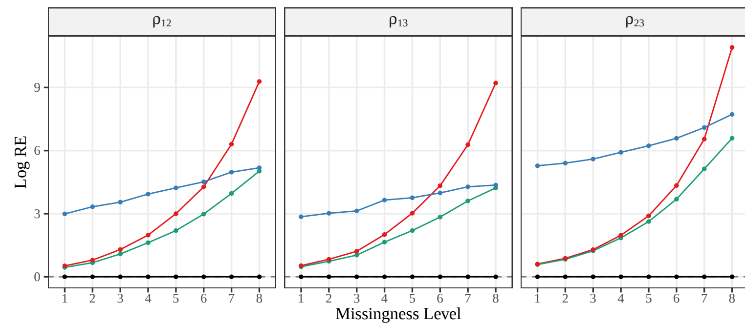
Correlation: Log RE
