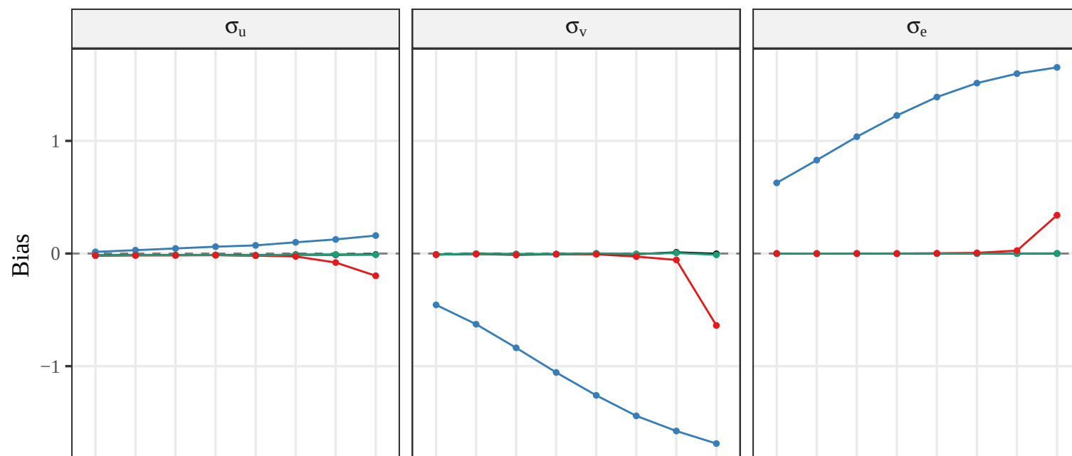
Variance Comp: Bias
