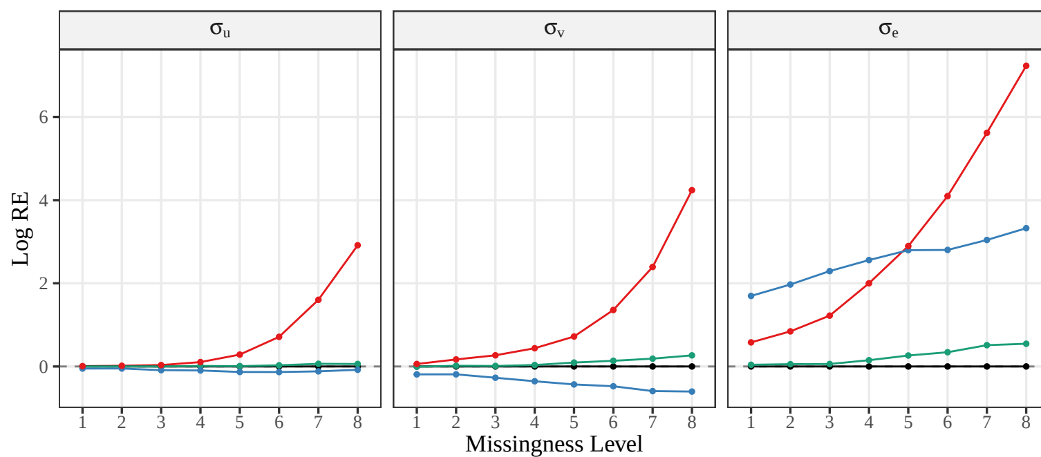
Variance Comp: Log RE
